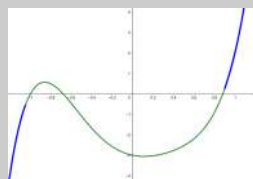
g(x)
